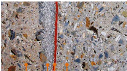
Secondary sprayed or cast concrete lining TamSeal 800 – 1 st coat orange, 2 nd coat grey Regulating layer such as TamCrete TopShot Primary sprayed concrete lining
